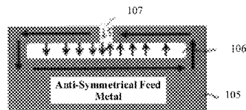
(c) Slot CM
