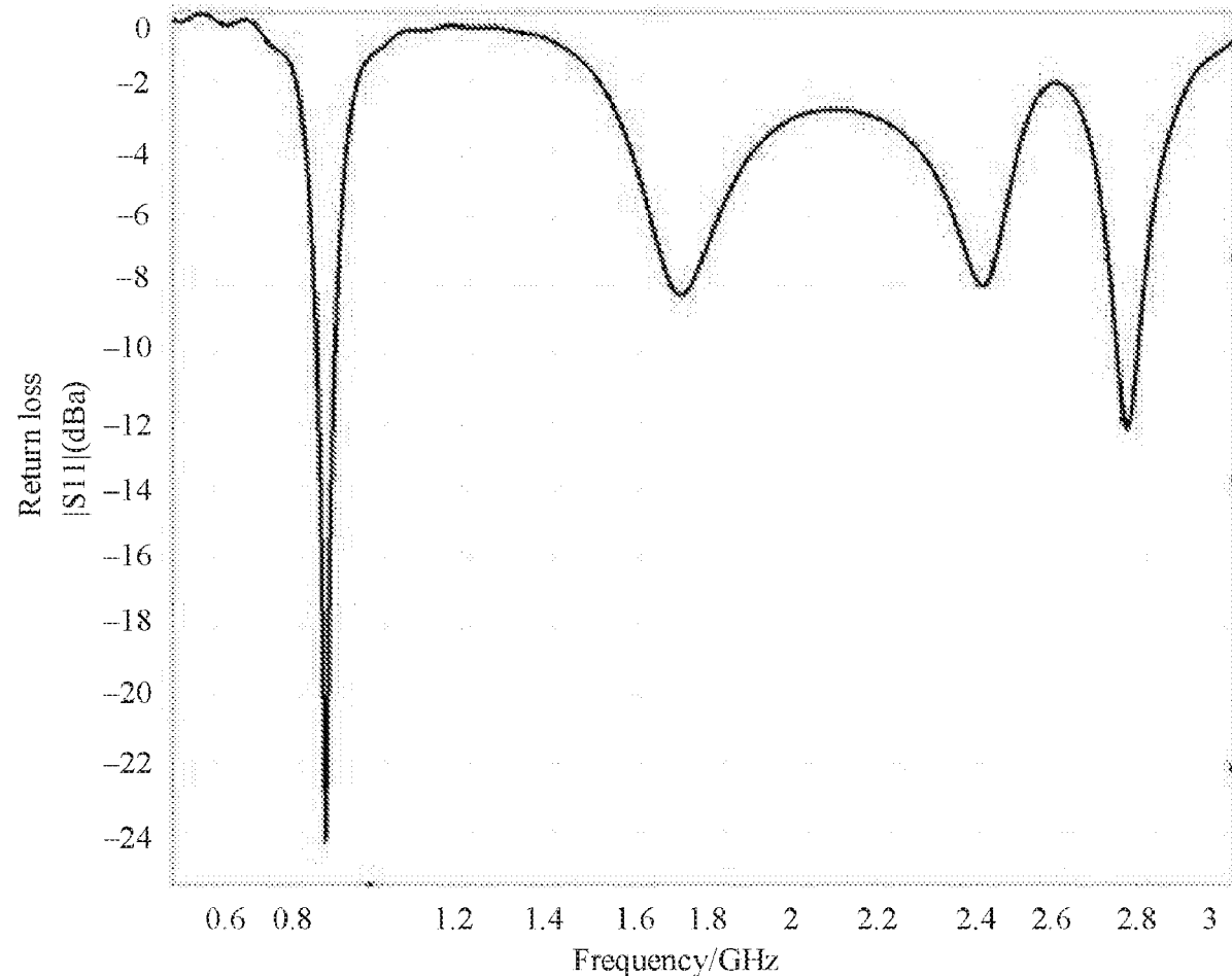
Relationship between a return loss and a frequency
