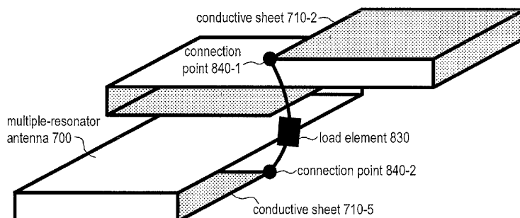
Multiple-resonator antenna with load element 800
